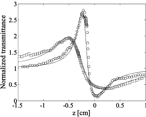
FIGURE 8 Calculated Z-scan curves for different focusing lenses with m = 3 . The parameters were c_+ = 1.6 \times 10 ; c_- = -1.4 \times 10^7 ; input polarization of 0^\circ and the following beam waists: 17 \mu\text{m} (black), and 30 \mu\text{m} (gray). Symbols are the experimental results for focal length lenses of: 3.5 cm (circles) and 6 cm (squares).
